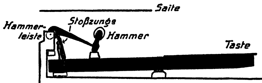
FIGURE 125. German Stossmechanik with escapement; del. Carmina Manger.
